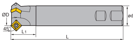
Weldon shank
