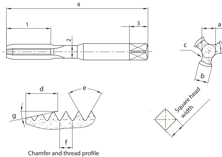
Chamfer and thread profile
